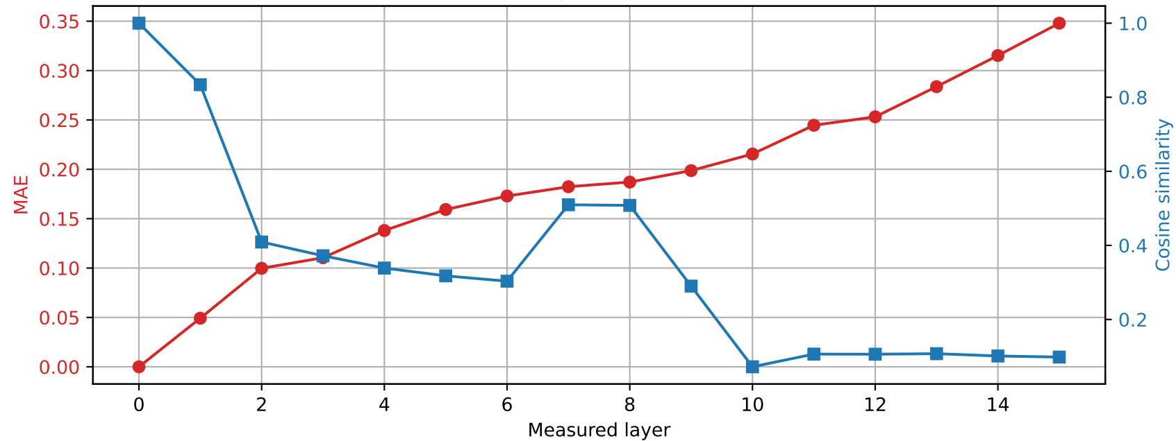
OLMo-1B-hf | Prompt 2 Spared layer 14 | Hybrid vs unquantized
