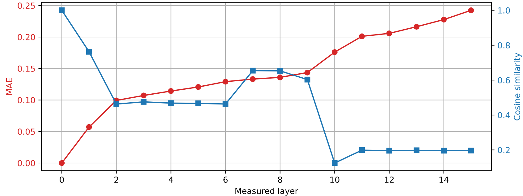
OLMo-1B-hf | Prompt 3 Spared layer 3 | Hybrid vs unquantized
