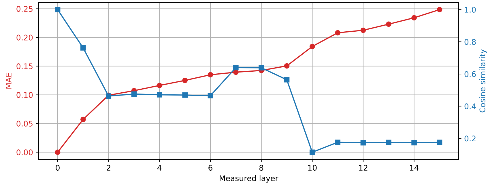
OLMo-1B-hf | Prompt 3 Spared layer 14 | Hybrid vs unquantized
