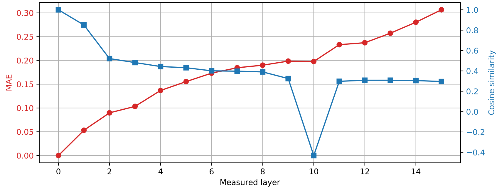
OLMo-1B-hf | Prompt 4 Unquantized vs quantized int4
