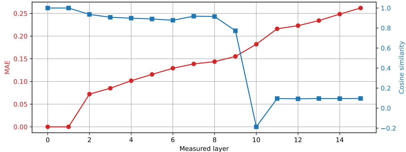
OLMo-1B-hf | Prompt 4 Spared layer 0 | Hybrid vs unquantized
