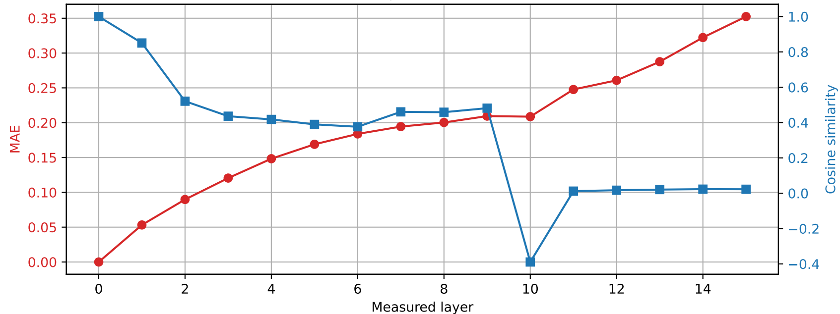
OLMo-1B-hf | Prompt 4 Spared layer 2 | Hybrid vs unquantized
