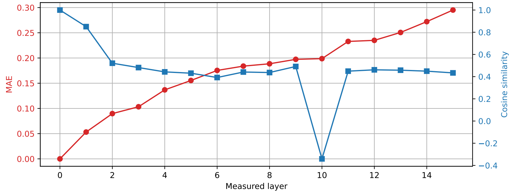
OLMo-1B-hf | Prompt 4 Spared layer 5 | Hybrid vs unquantized
