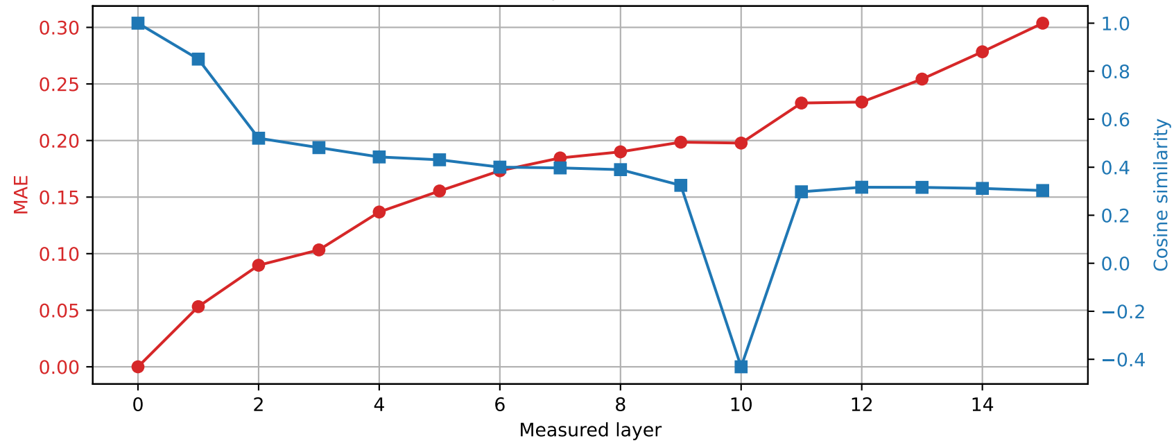
OLMo-1B-hf | Prompt 4 Spared layer 11 | Hybrid vs unquantized
