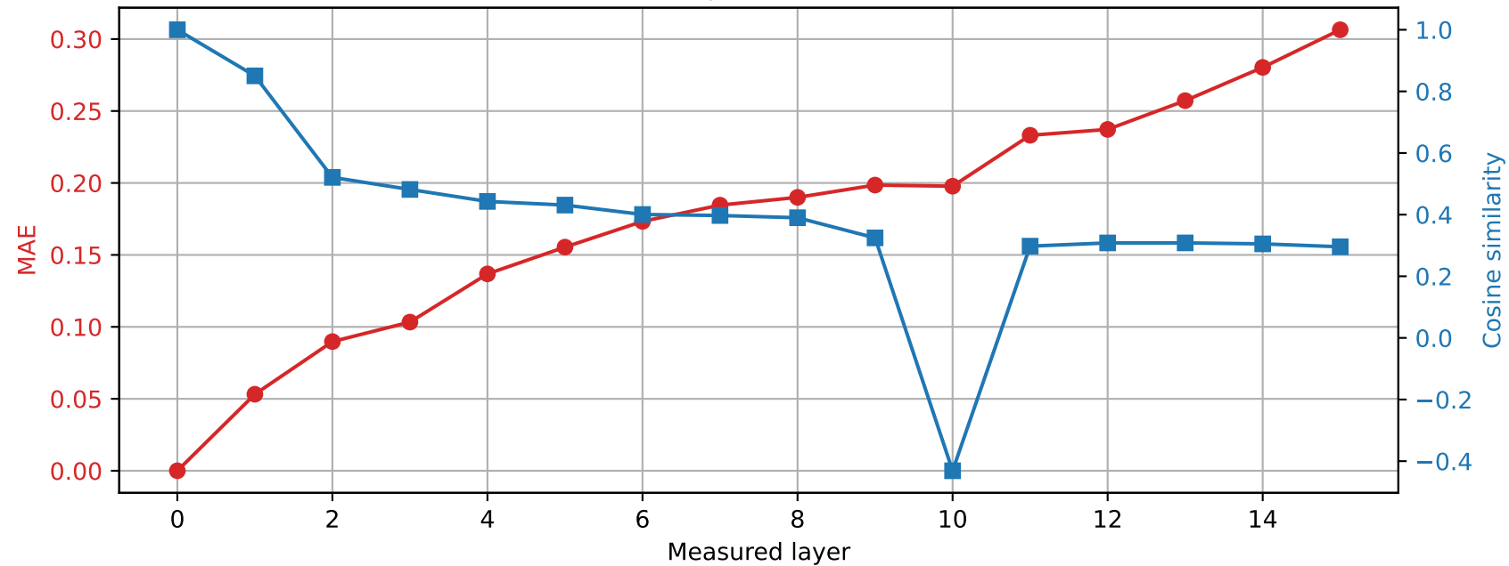
OLMo-1B-hf | Prompt 4 Spared layer 15 | Hybrid vs unquantized
