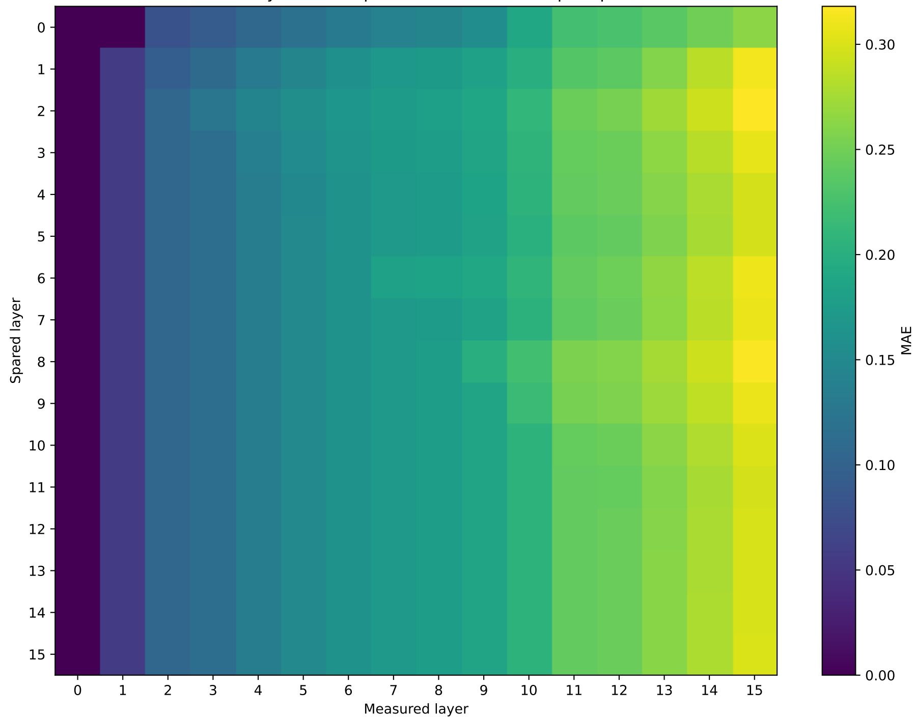
OLMo-1B-hf Mean hybrid vs unquantized MAE across 5 prompts
