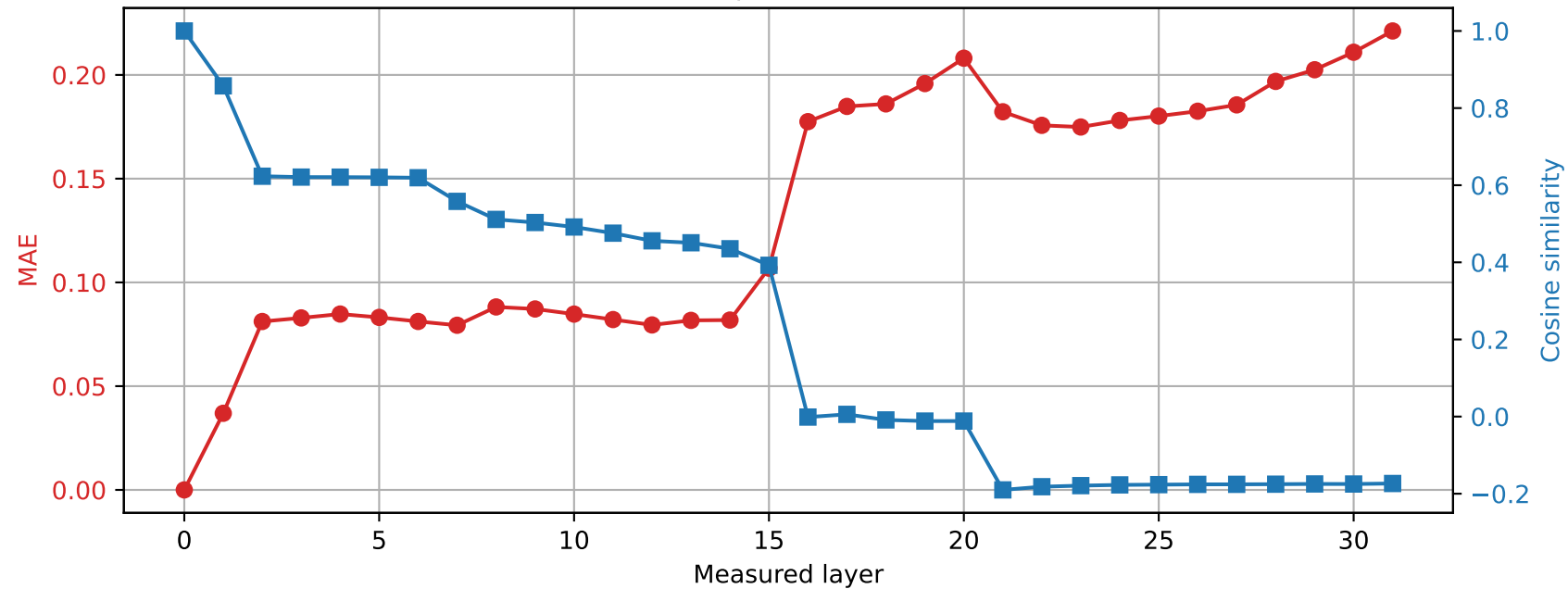
OLMo-7B-hf | Prompt 0 Spared layer 11 | Hybrid vs unquantized
