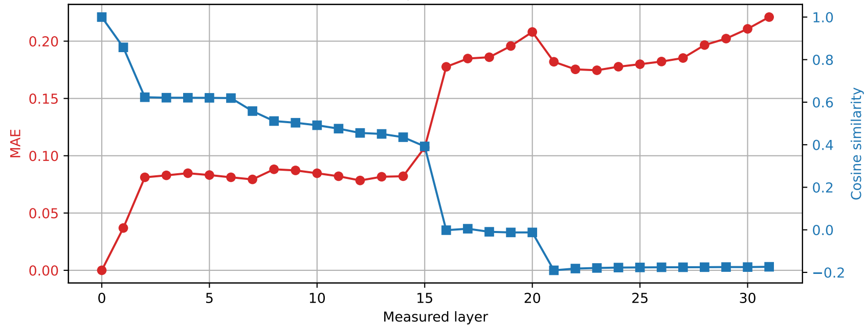
OLMo-7B-hf | Prompt 0 Spared layer 12 | Hybrid vs unquantized
