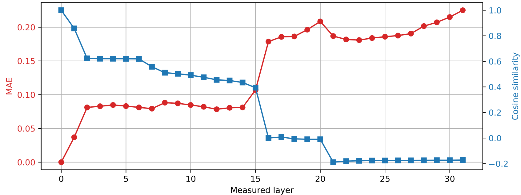
OLMo-7B-hf | Prompt 0 Spared layer 14 | Hybrid vs unquantized
