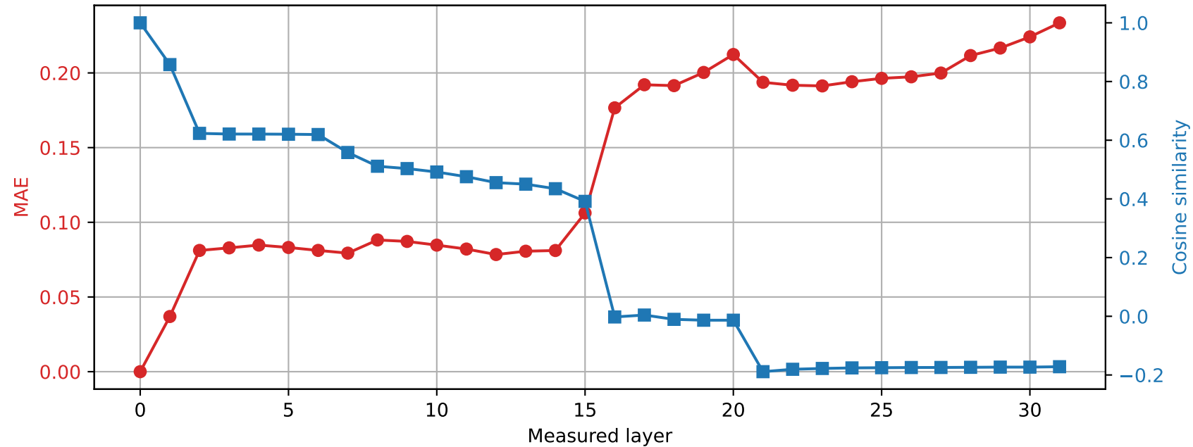
OLMo-7B-hf | Prompt 0 Spared layer 16 | Hybrid vs unquantized
