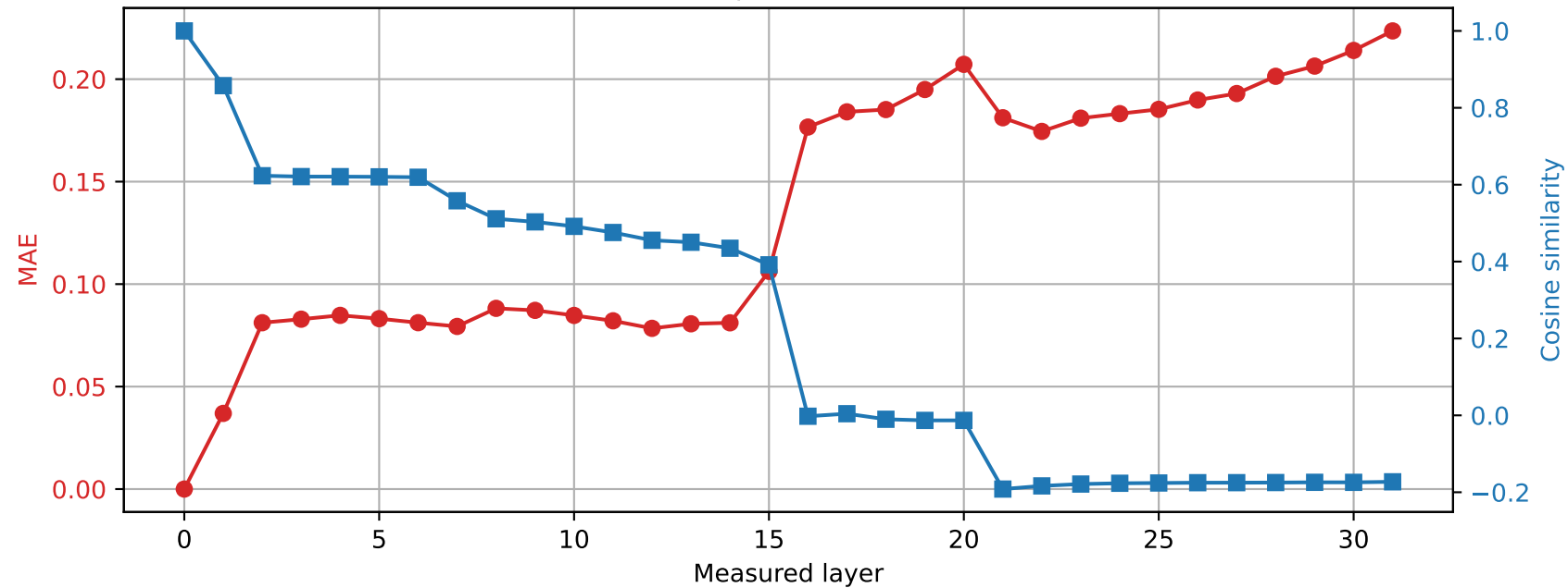
OLMo-7B-hf | Prompt 0 Spared layer 22 | Hybrid vs unquantized
