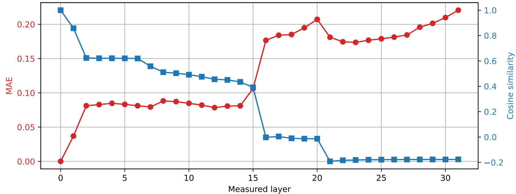
OLMo-7B-hf | Prompt 0 Spared layer 30 | Hybrid vs unquantized
