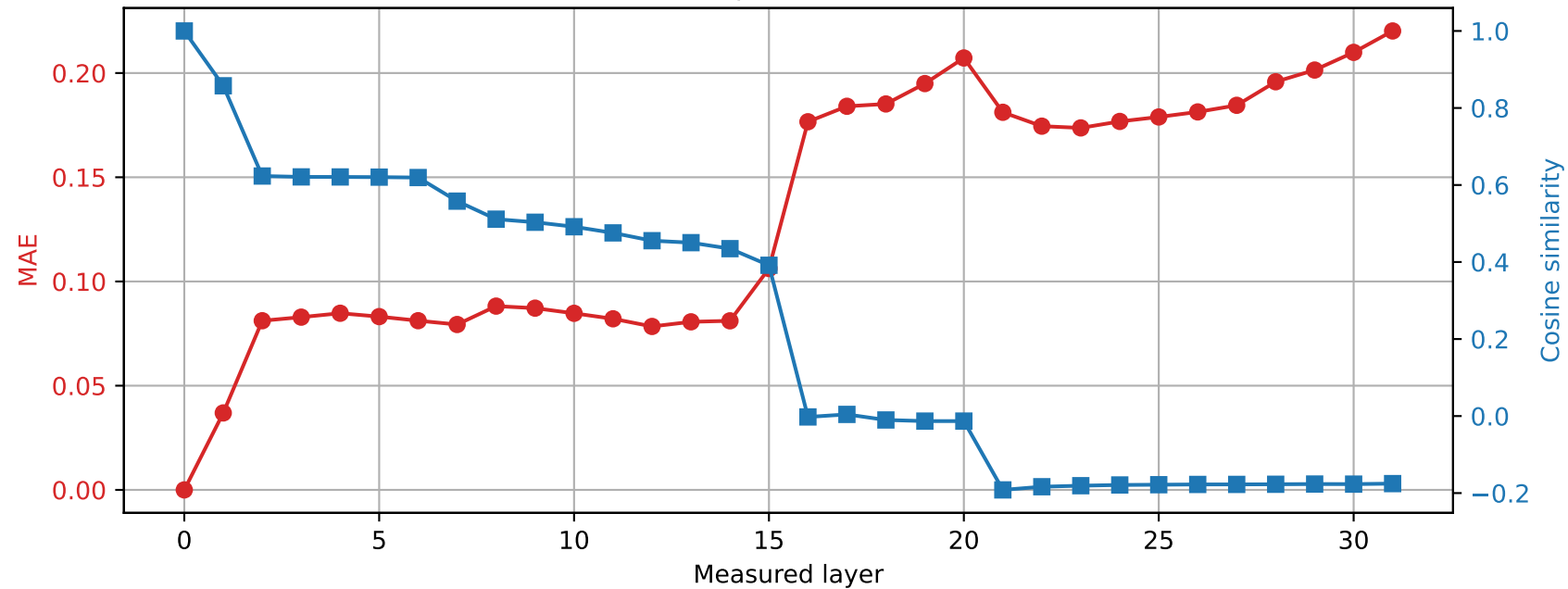
OLMo-7B-hf | Prompt 0 Spared layer 31 | Hybrid vs unquantized
