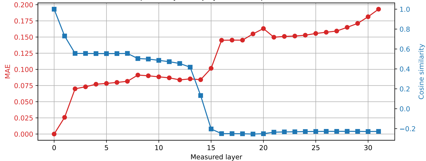
OLMo-7B-hf | Prompt 1 Spared layer 18 | Hybrid vs unquantized
