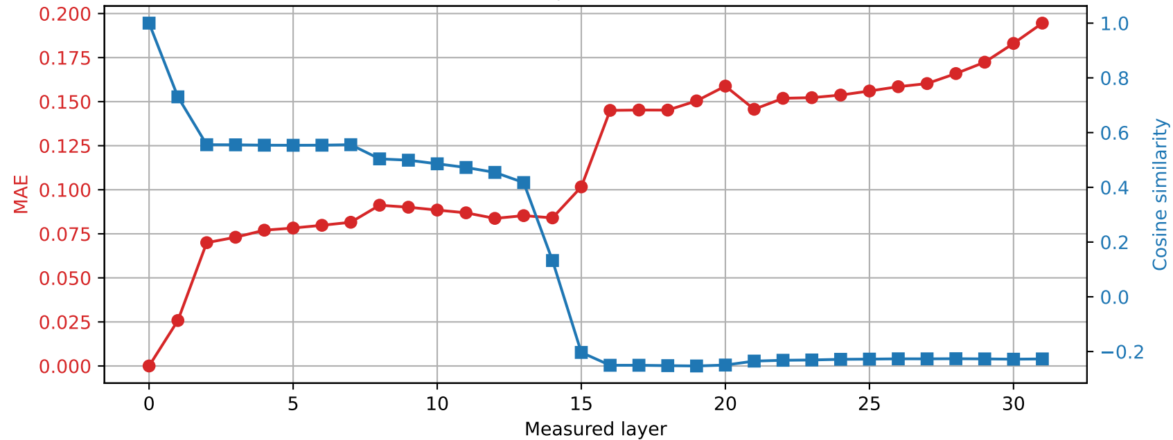
OLMo-7B-hf | Prompt 1 Spared layer 21 | Hybrid vs unquantized
