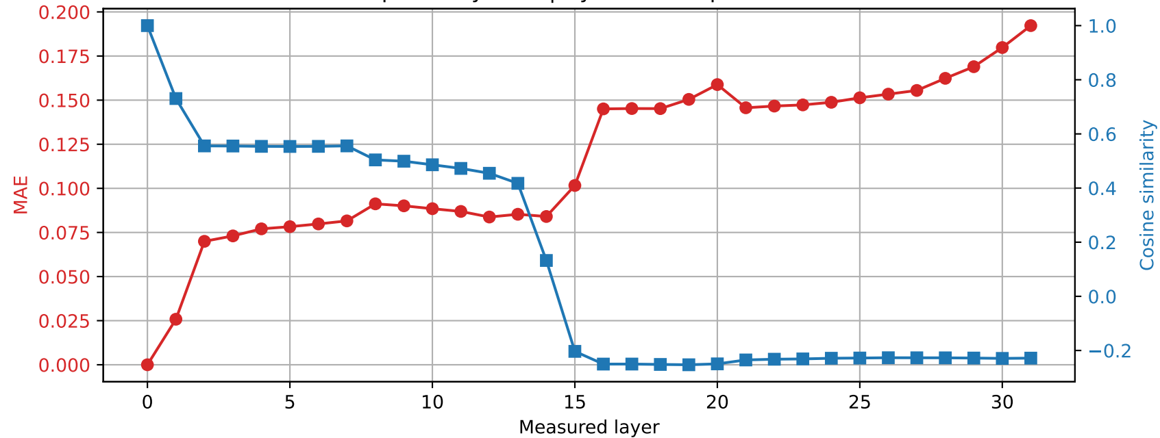
OLMo-7B-hf | Prompt 1 Spared layer 27 | Hybrid vs unquantized
