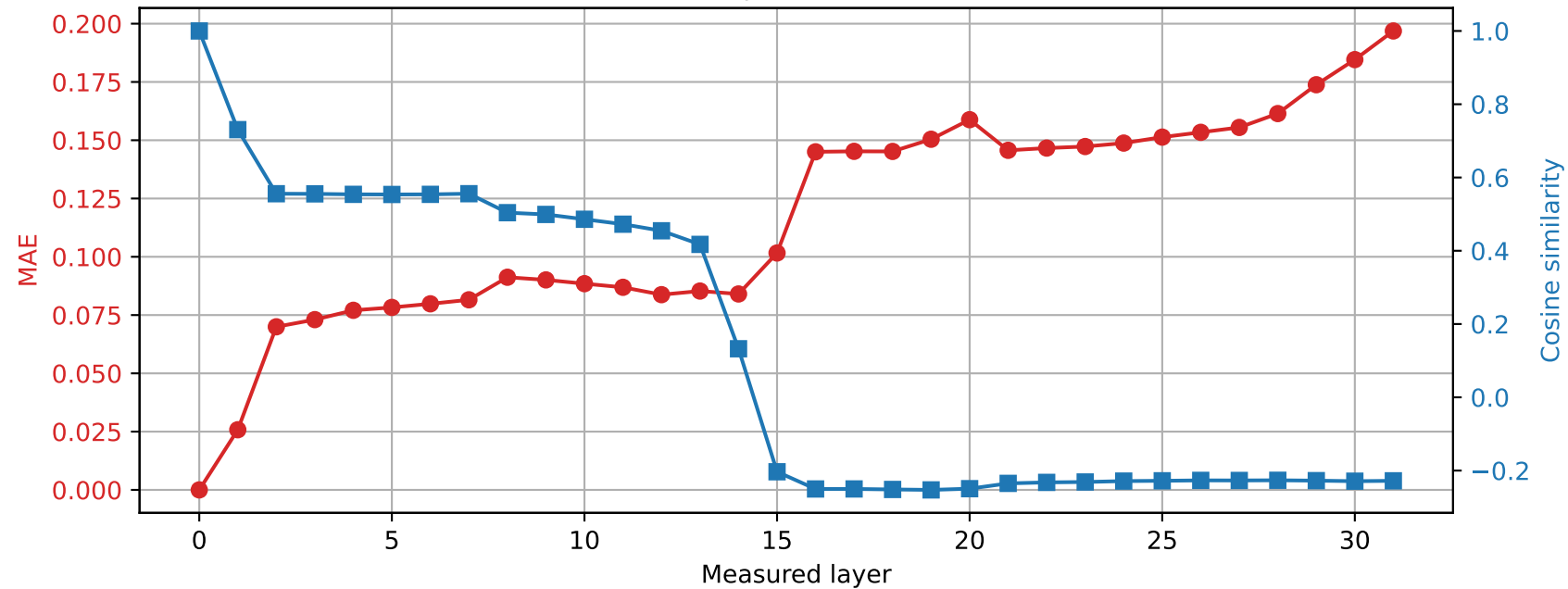
OLMo-7B-hf | Prompt 1 Spared layer 28 | Hybrid vs unquantized
