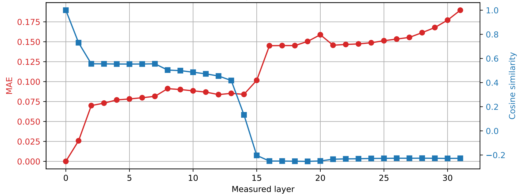
OLMo-7B-hf | Prompt 1 Spared layer 29 | Hybrid vs unquantized
