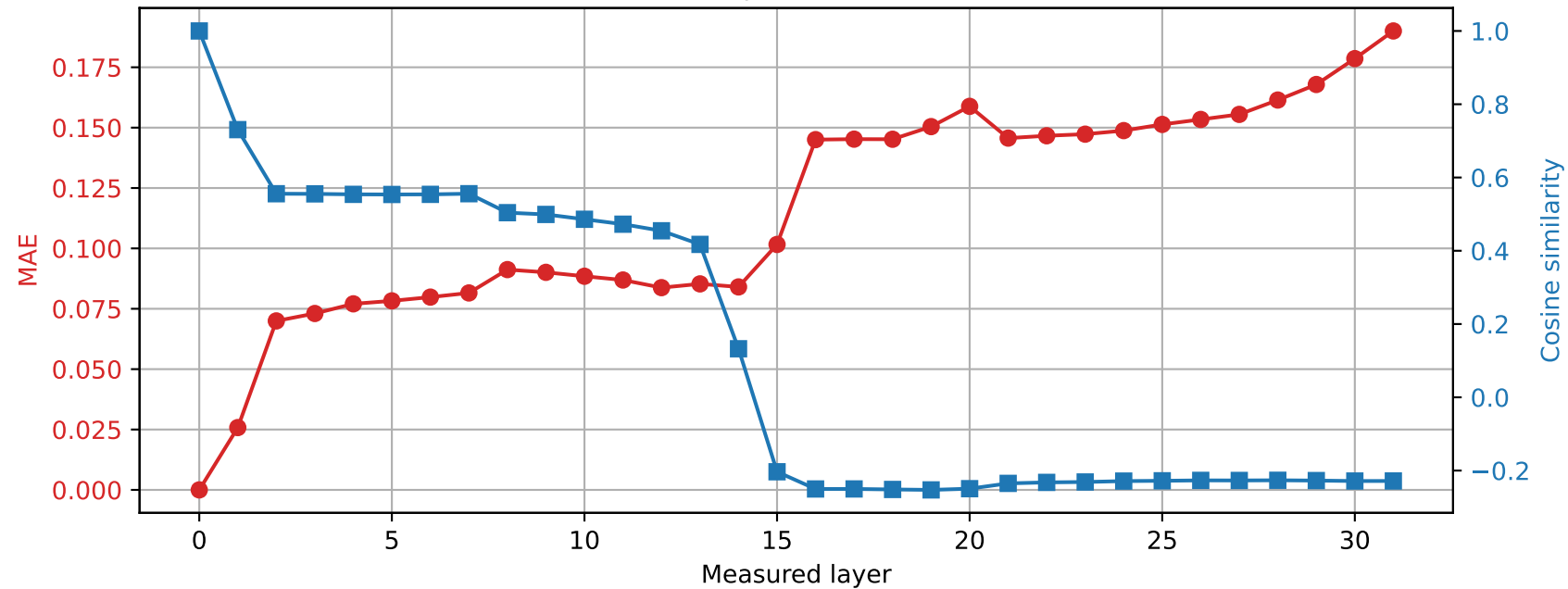
OLMo-7B-hf | Prompt 1 Spared layer 30 | Hybrid vs unquantized
