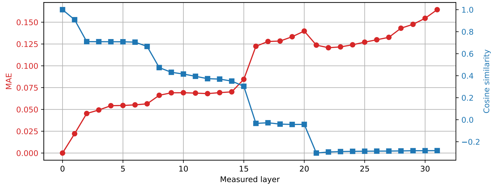
OLMo-7B-hf | Prompt 2 Spared layer 3 | Hybrid vs unquantized
