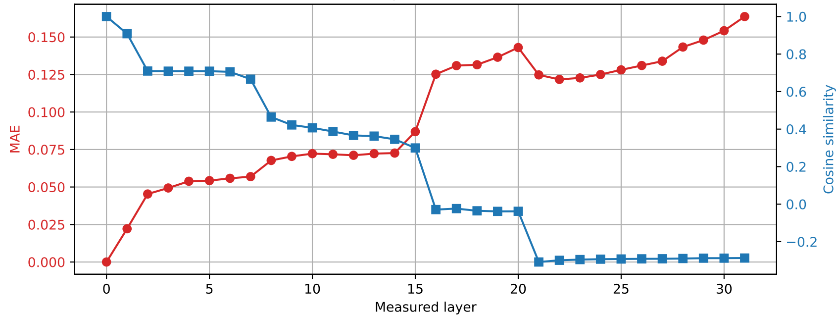
OLMo-7B-hf | Prompt 2 Spared layer 9 | Hybrid vs unquantized
