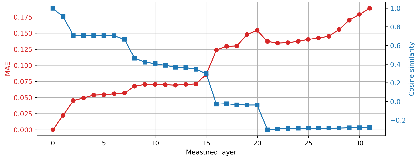
OLMo-7B-hf | Prompt 2 Spared layer 18 | Hybrid vs unquantized
