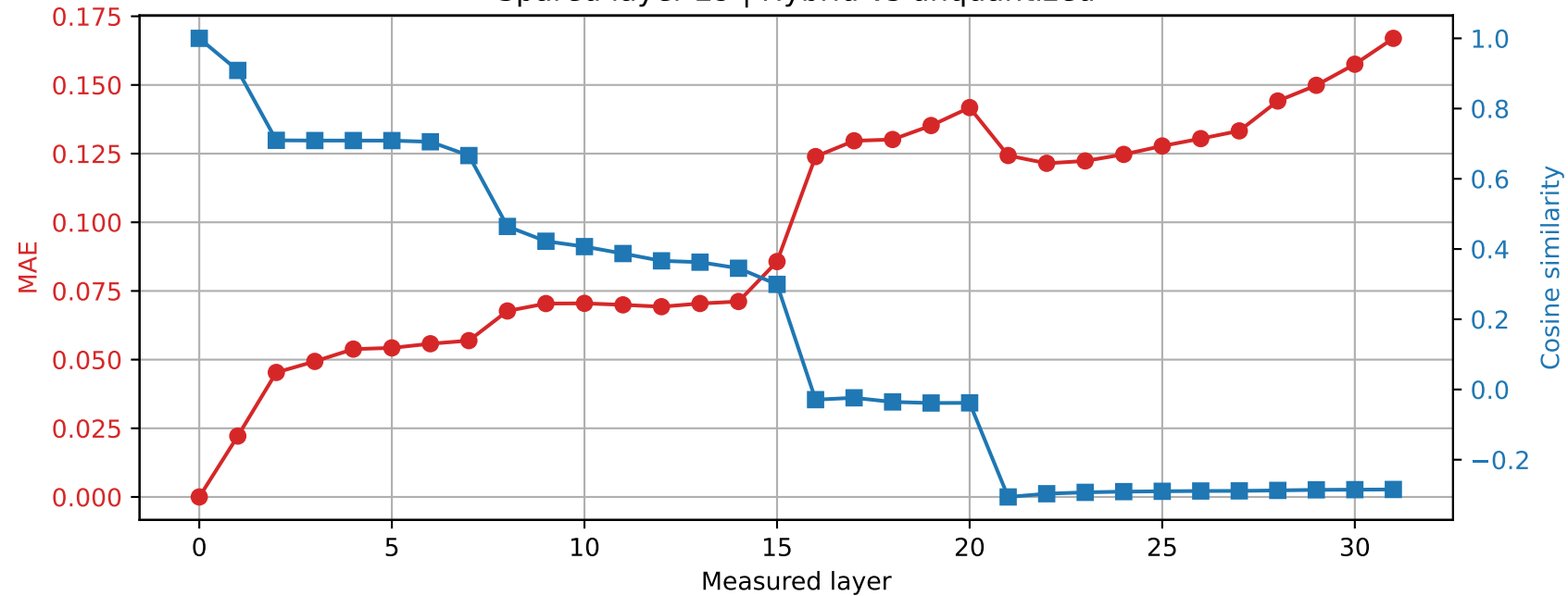
OLMo-7B-hf | Prompt 2 Spared layer 29 | Hybrid vs unquantized
