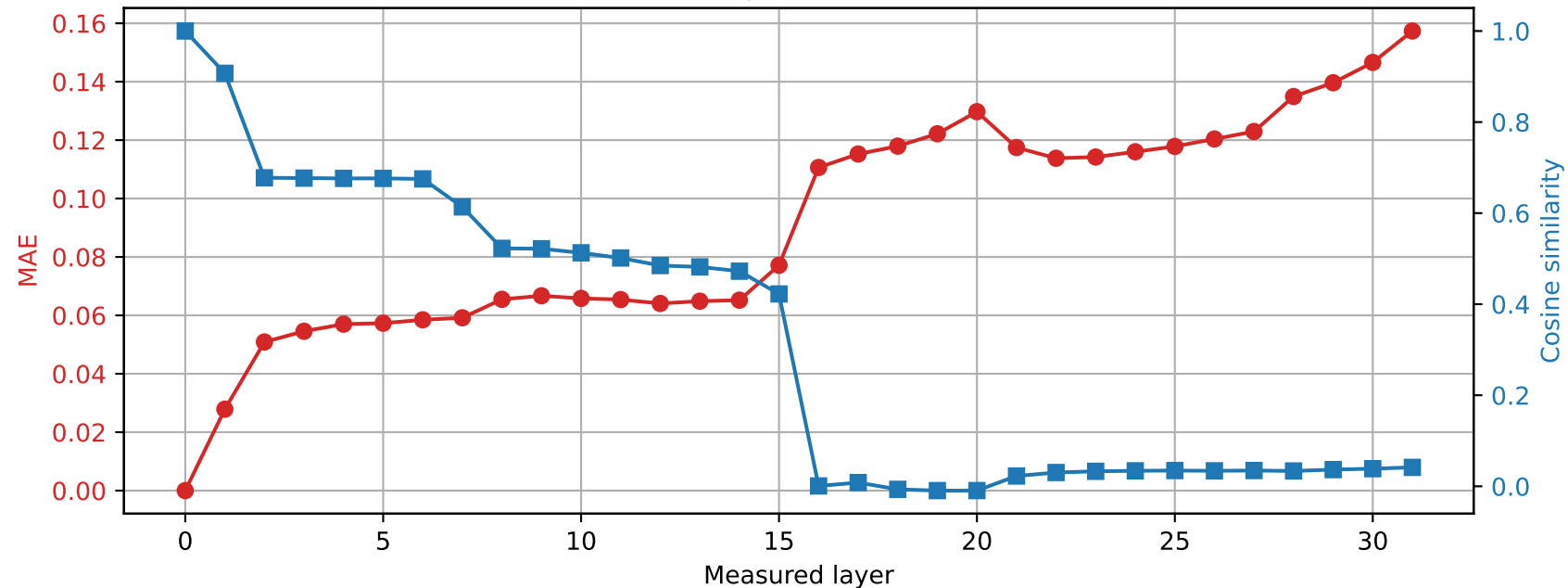
OLMo-7B-hf | Prompt 3 Spared layer 10 | Hybrid vs unquantized
