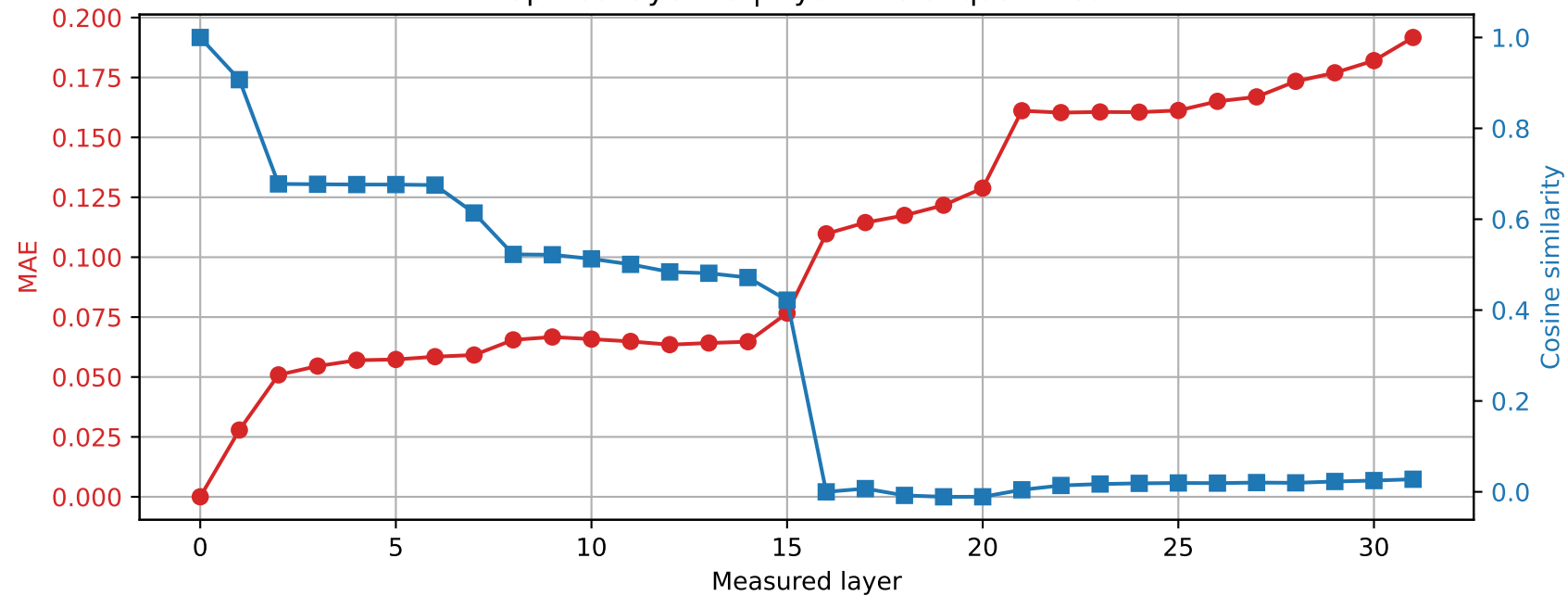
OLMo-7B-hf | Prompt 3 Spared layer 20 | Hybrid vs unquantized
