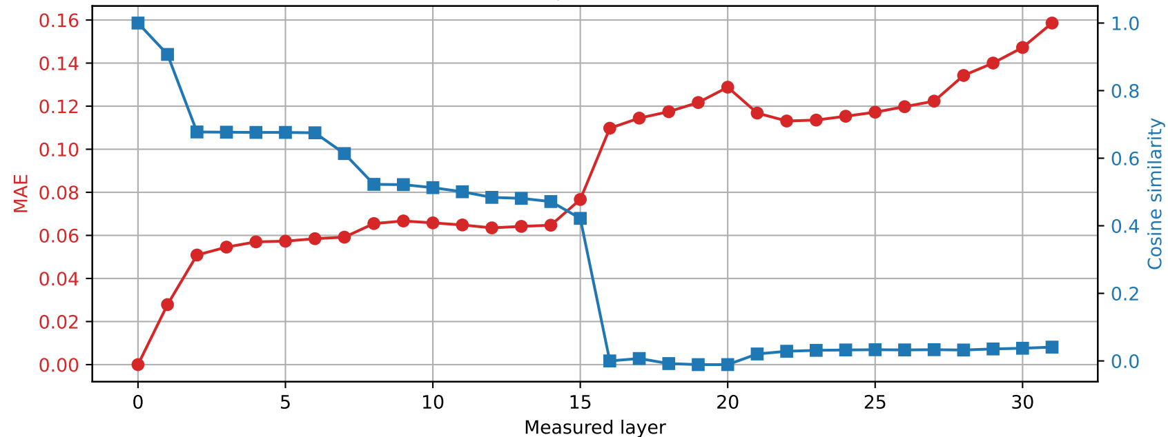
OLMo-7B-hf | Prompt 3 Spared layer 30 | Hybrid vs unquantized
