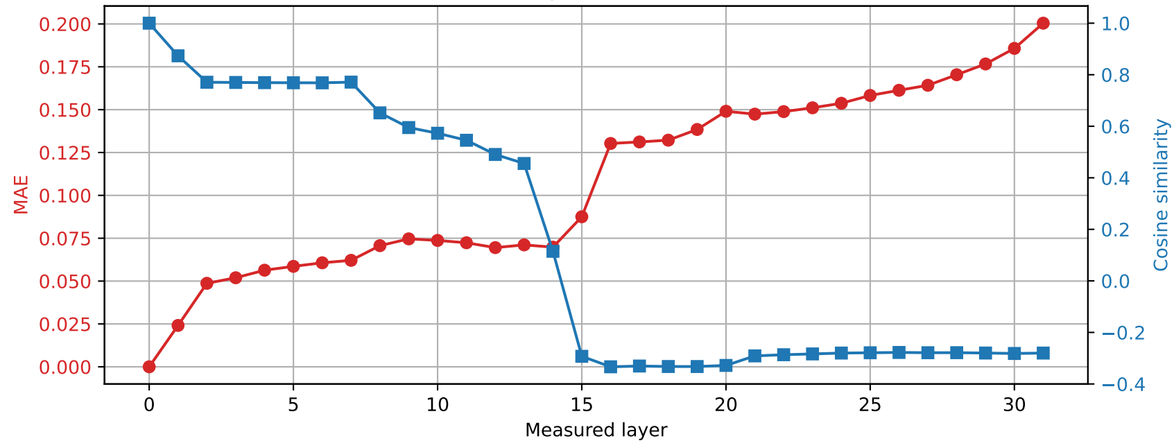
OLMo-7B-hf | Prompt 4 Spared layer 5 | Hybrid vs unquantized
