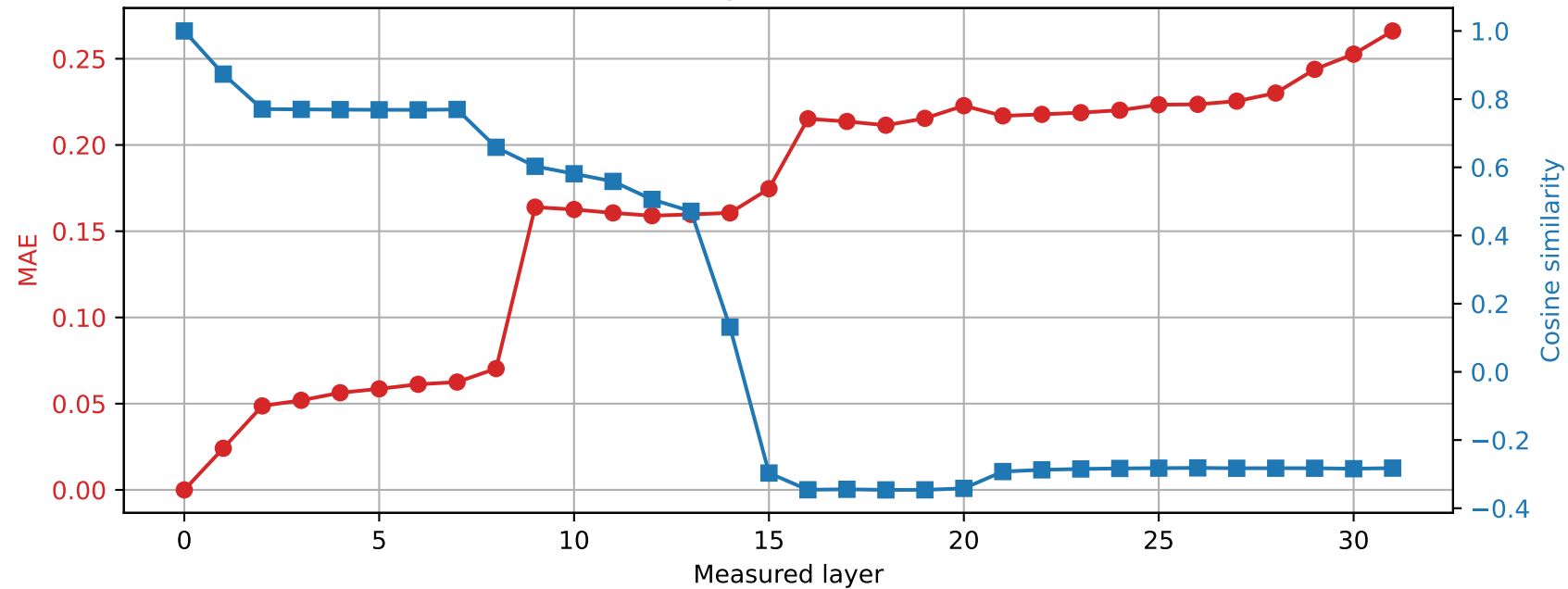
OLMo-7B-hf | Prompt 4 Spared layer 8 | Hybrid vs unquantized
