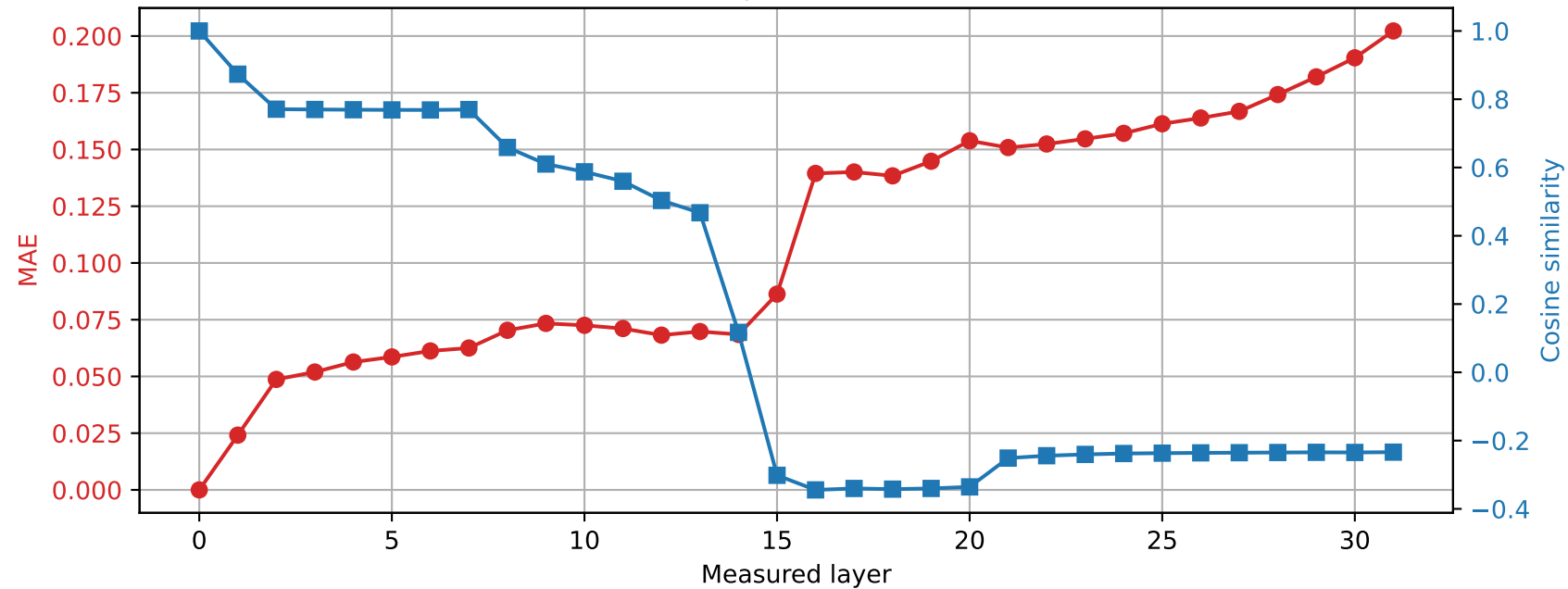
OLMo-7B-hf | Prompt 4 Spared layer 15 | Hybrid vs unquantized
