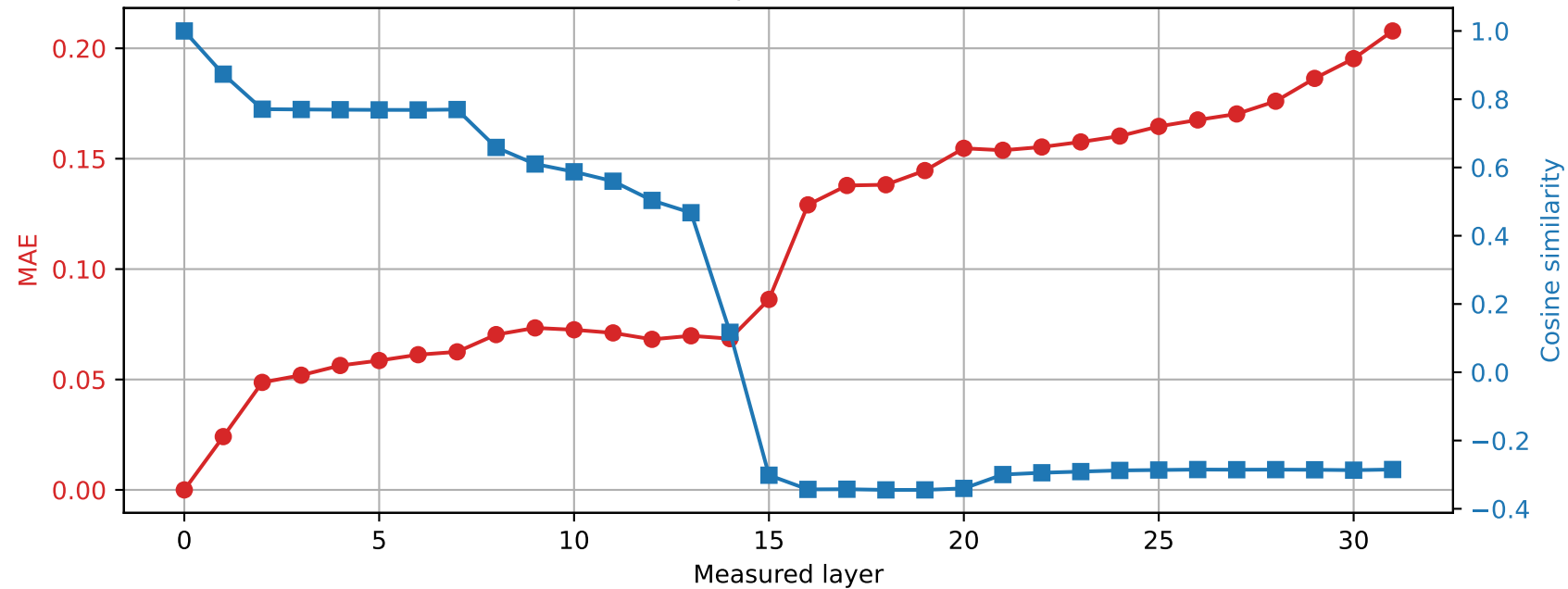
OLMo-7B-hf | Prompt 4 Spared layer 16 | Hybrid vs unquantized
