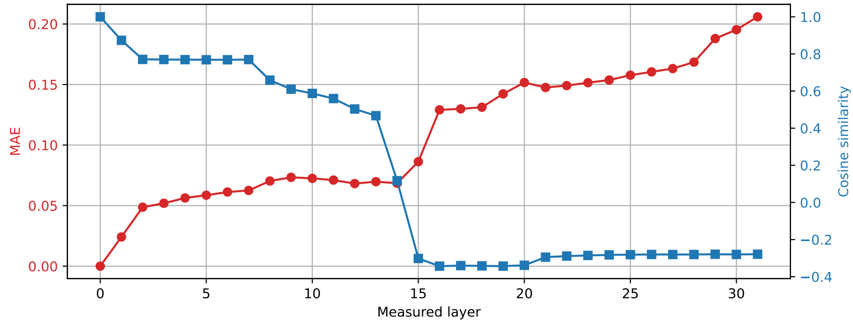
OLMo-7B-hf | Prompt 4 Spared layer 18 | Hybrid vs unquantized
