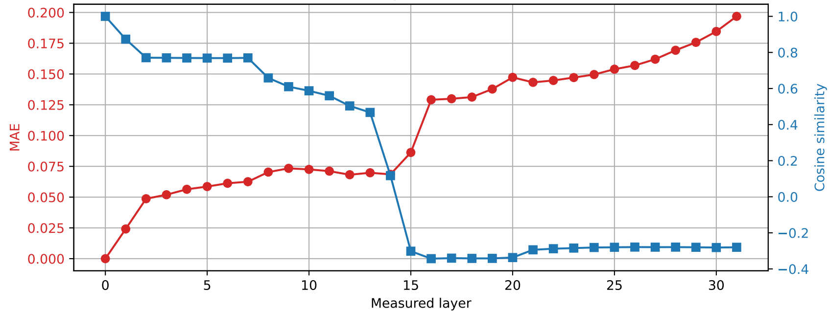
OLMo-7B-hf | Prompt 4 Spared layer 26 | Hybrid vs unquantized
