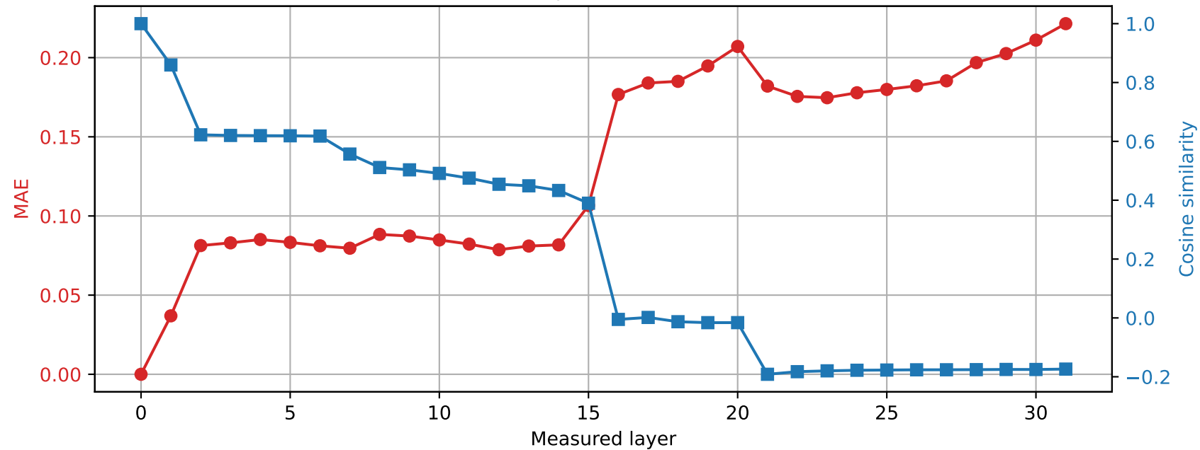
OLMo-7B-hf | Prompt 0 Spared layer 3 | Hybrid vs unquantized
