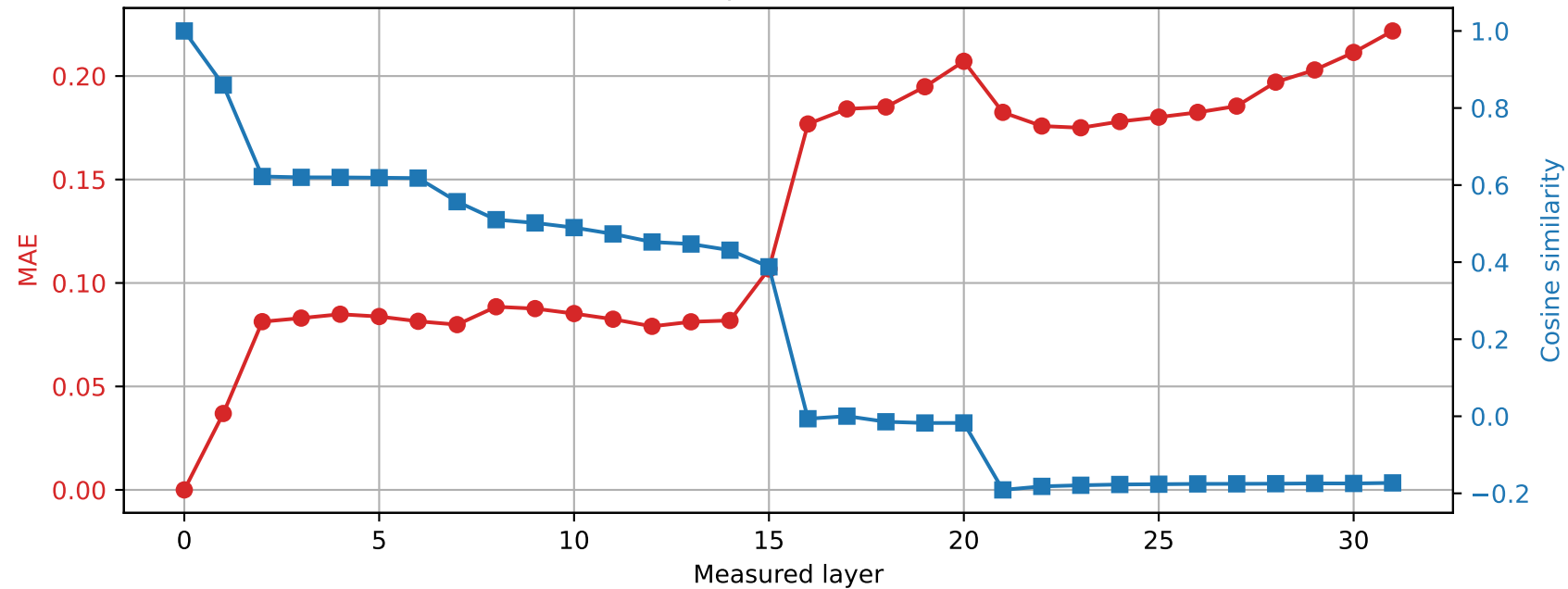
OLMo-7B-hf | Prompt 0 Spared layer 4 | Hybrid vs unquantized
