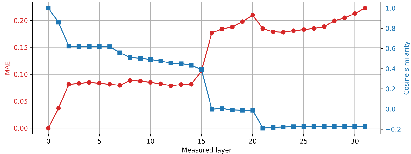
OLMo-7B-hf | Prompt 0 Spared layer 17 | Hybrid vs unquantized
