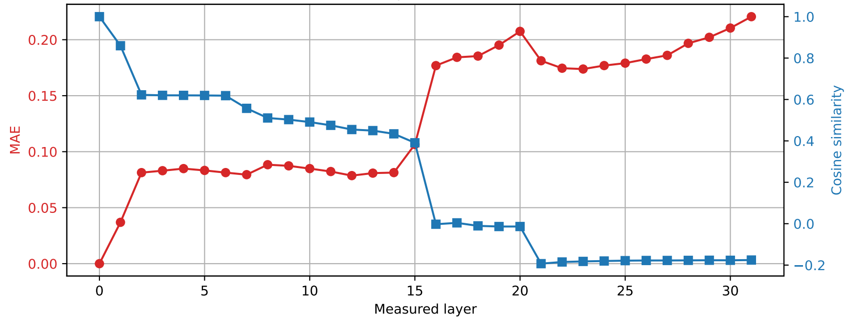
OLMo-7B-hf | Prompt 0 Spared layer 24 | Hybrid vs unquantized
