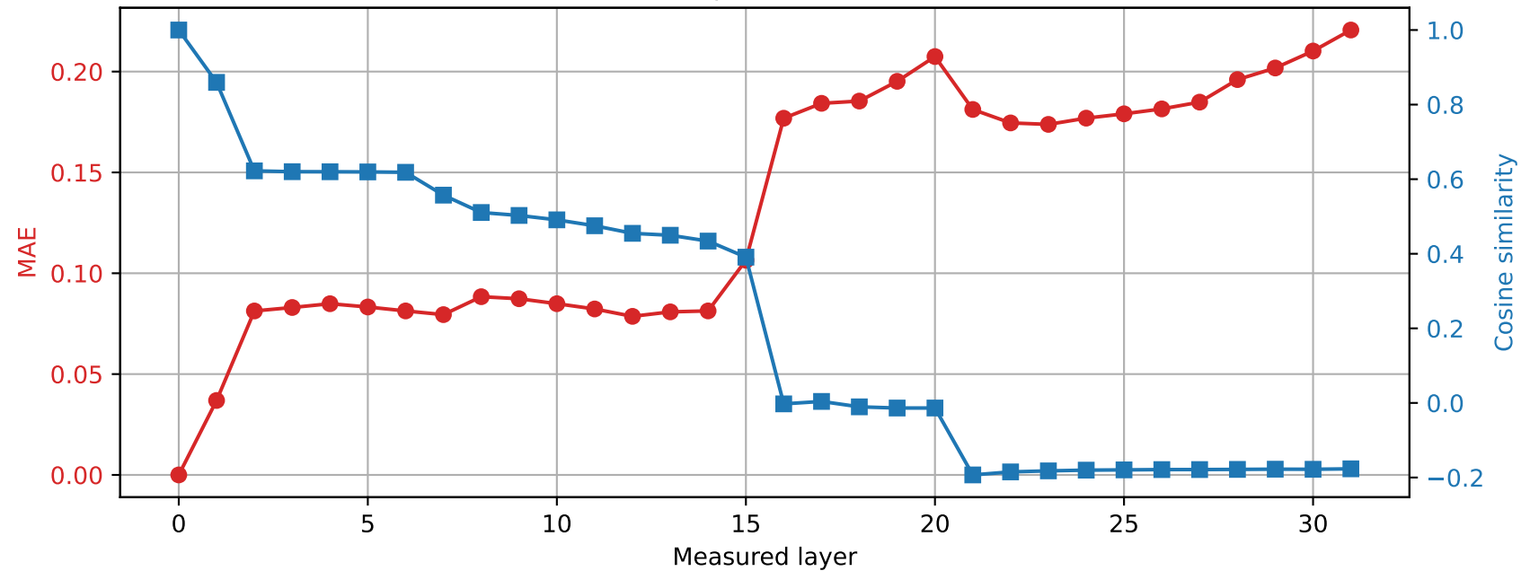
OLMo-7B-hf | Prompt 0 Spared layer 25 | Hybrid vs unquantized
