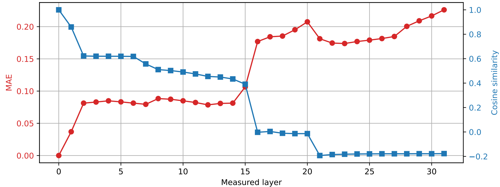
OLMo-7B-hf | Prompt 0 Spared layer 27 | Hybrid vs unquantized
