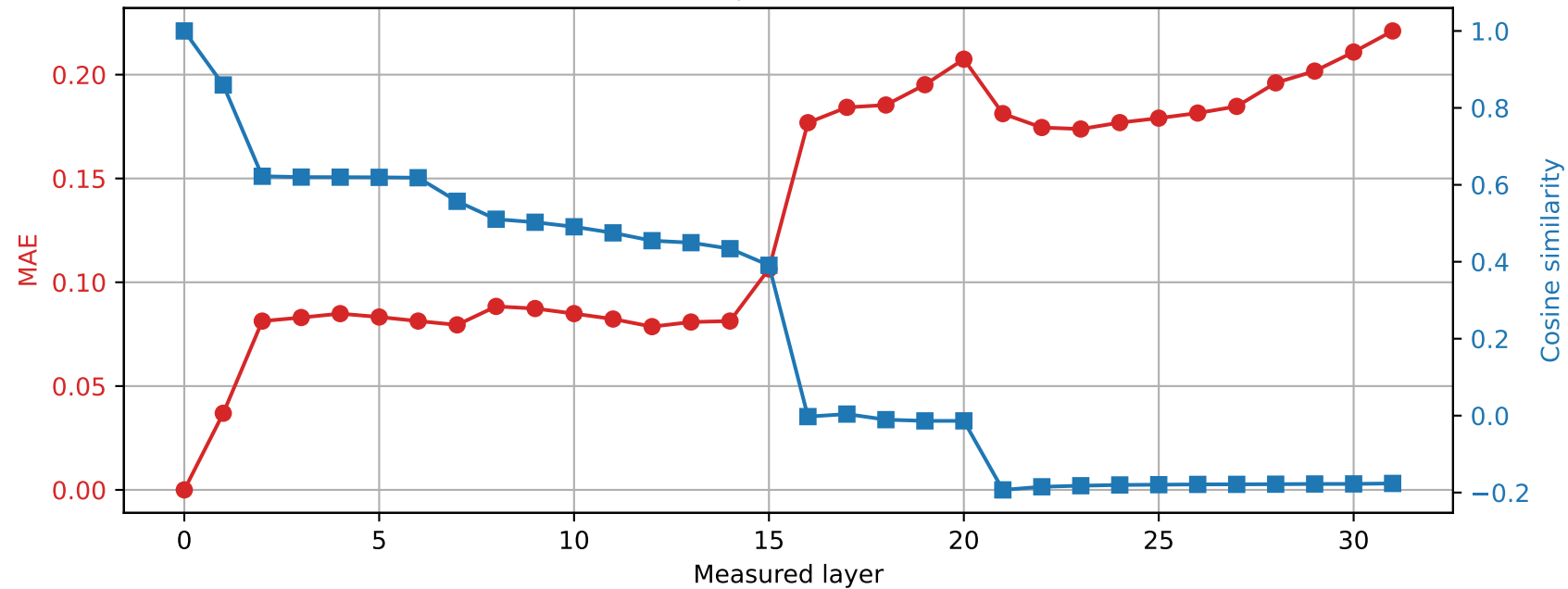
OLMo-7B-hf | Prompt 0 Spared layer 29 | Hybrid vs unquantized
