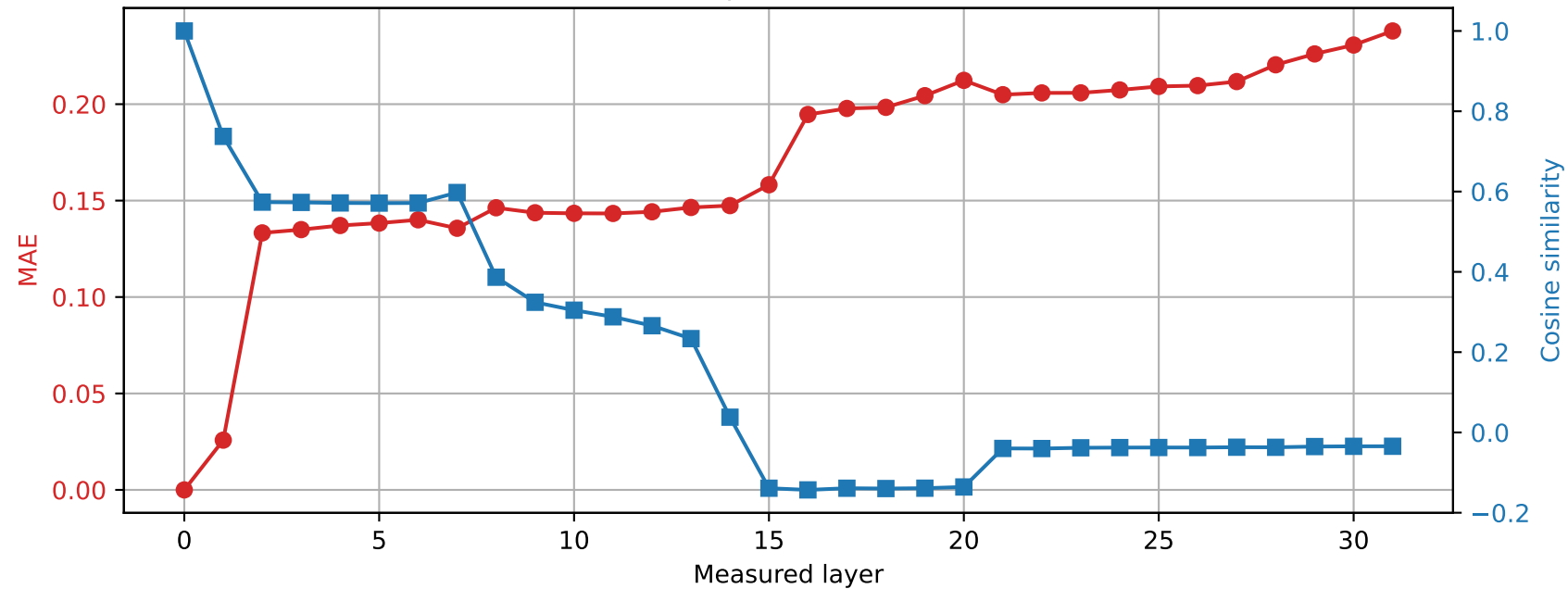
OLMo-7B-hf | Prompt 1 Spared layer 1 | Hybrid vs unquantized
