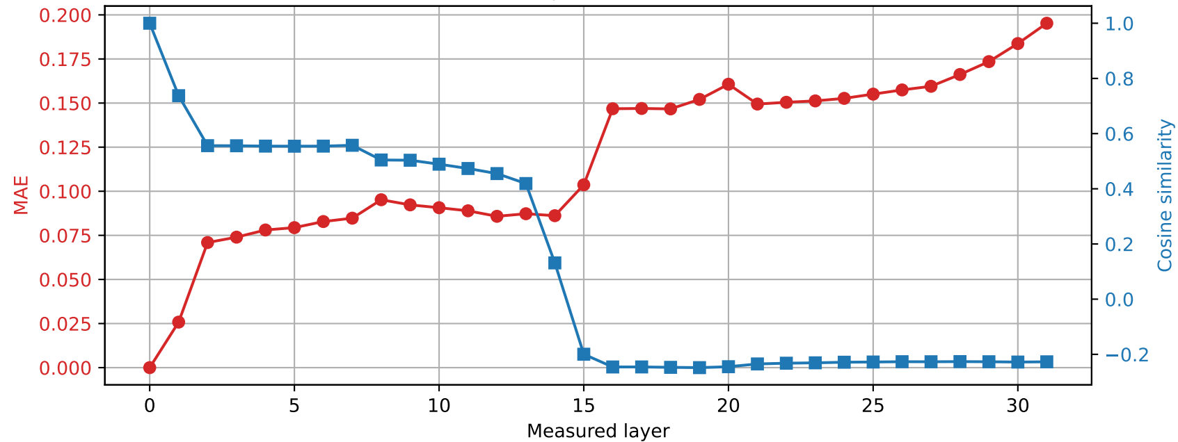
OLMo-7B-hf | Prompt 1 Spared layer 5 | Hybrid vs unquantized
