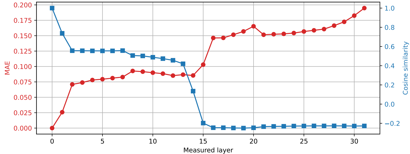
OLMo-7B-hf | Prompt 1 Spared layer 17 | Hybrid vs unquantized
