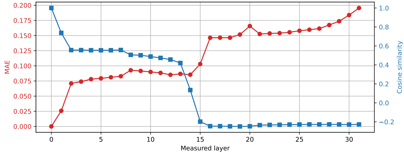
OLMo-7B-hf | Prompt 1 Spared layer 19 | Hybrid vs unquantized
