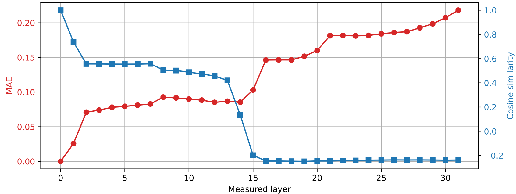
OLMo-7B-hf | Prompt 1 Spared layer 20 | Hybrid vs unquantized
