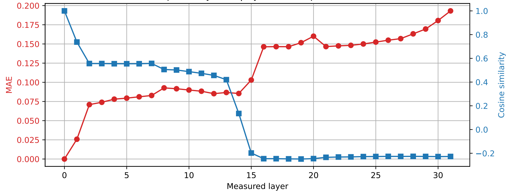
OLMo-7B-hf | Prompt 1 Spared layer 23 | Hybrid vs unquantized
