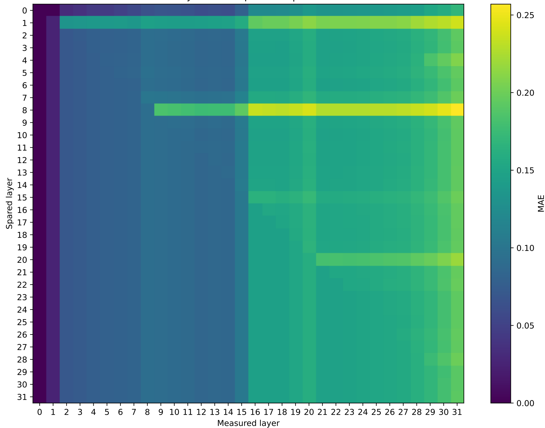
OLMo-7B-hf | Prompt 1 Hybrid vs unquantized | int4
